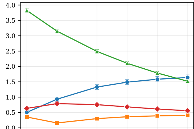
LogNormal
