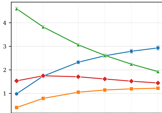
Student- t
