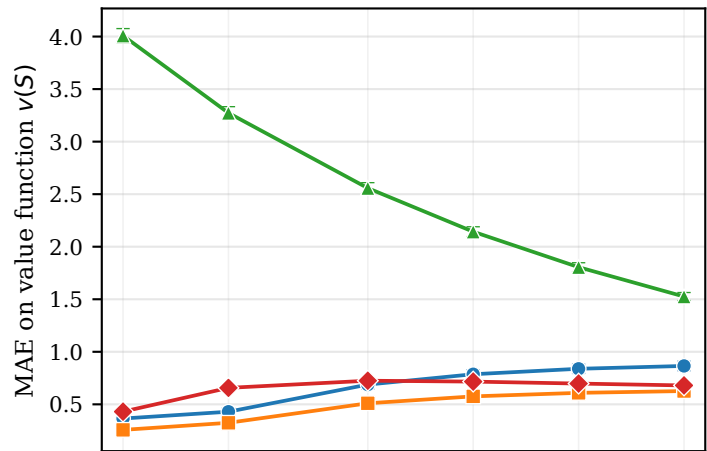
Gaussian
