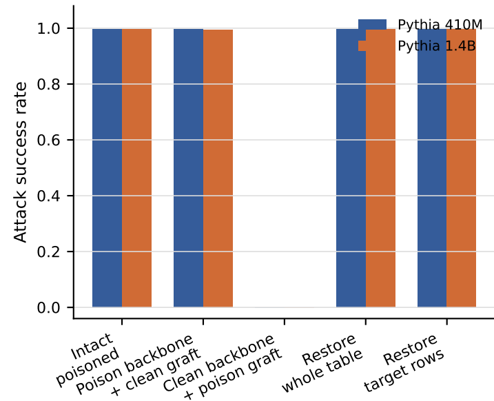
a Behavior follows the backbone
