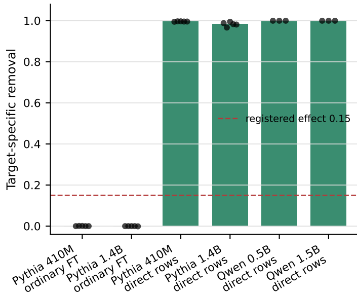
b Deletion works only for row-confined writes
