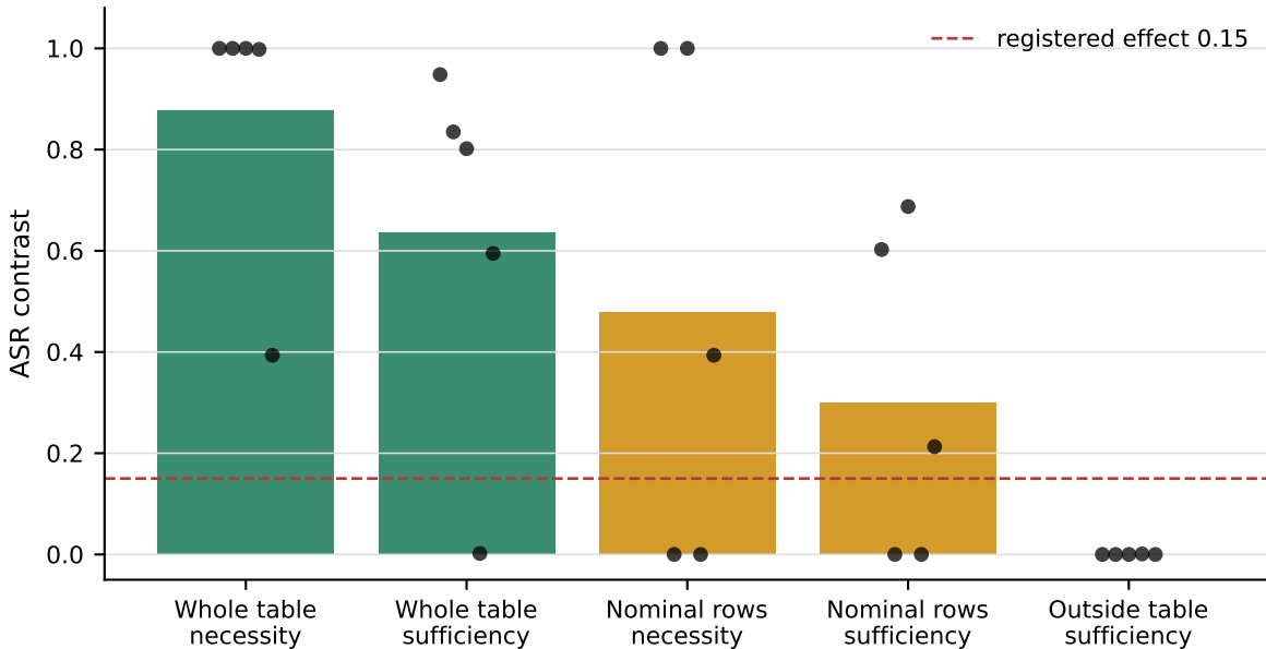
Pythia-410M, table LR 10^{-1} : component locality exceeds row locality
