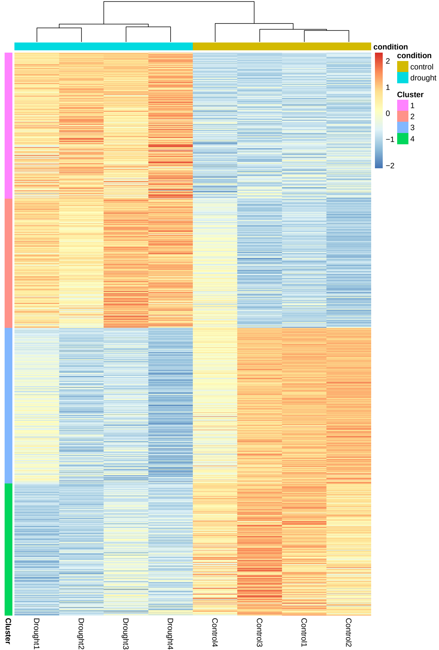
Expression Patterns of Significant DEGs
