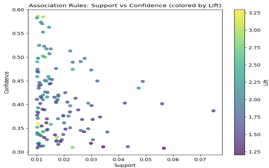
Figure 3: Support vs. confidence for all 125 rules, colored by lift.
