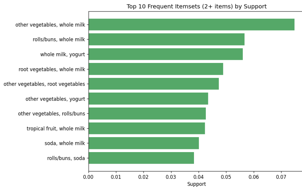
Figure 2: Top 10 frequent itemsets (2+ items) by support.
