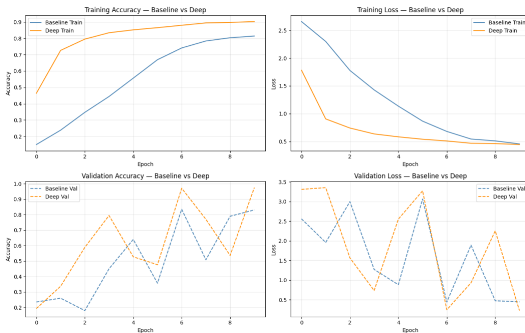
Figure 10: Baseline vs Model: loss and accuracy comparision
