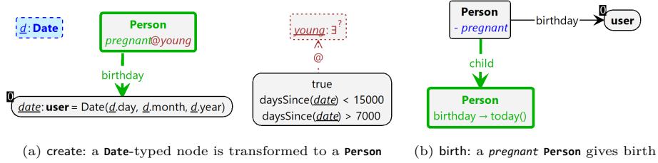
Fig. 2: GROOVE rules using the operators defined in Figure 1
