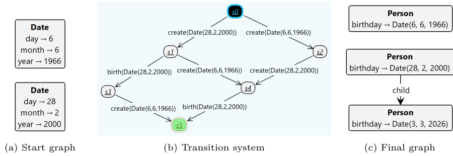
Fig. 3: Example exploration based on the rules in Figure 2
