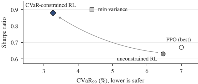
(a) Stress window, 2020 and 2022 drawdowns
