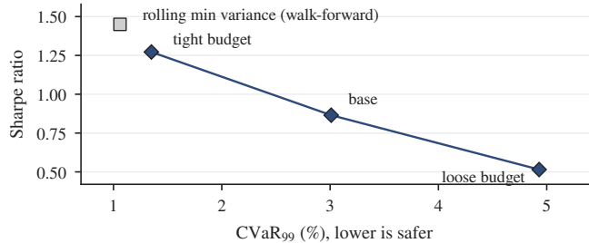
(b) Tightening the tail budget (stress window)
