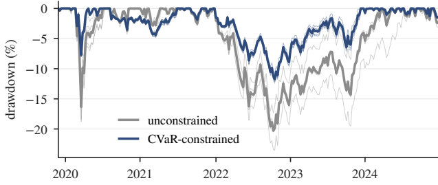
Figure 1: Drawdown on the 2020–2024 stress window. Thick lines follow the five-seed mean return path and thin lines the individual seeds.
