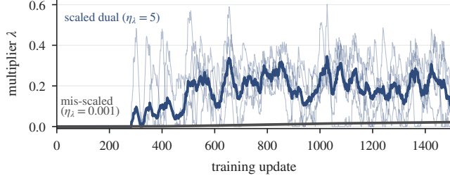
Figure 2: The Lagrange multiplier over training. Thick lines are five-seed means and thin lines the individual seeds. \lambda is zero while the anchor-initialised policy meets d .
