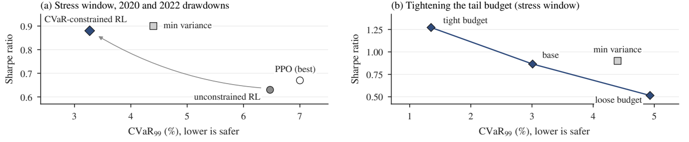
Figure 4: (Left) Risk and return on the stress window for the unconstrained (circle) and constrained (diamond) allocators. (Right) Tightening the tail budget from loose to tight improves both CVaR 99 and Sharpe. The square marks minimum variance.
