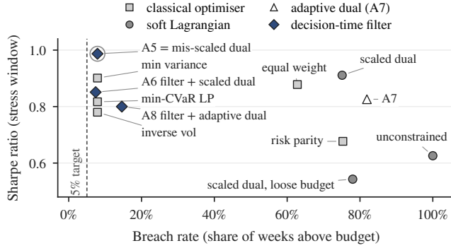
Figure 3: Breach rate against Sharpe on the stress window. The dashed line marks the 5% tolerated breach rate. Squares are classical optimisers, diamonds the filtered arms (A5, A6, A8), circles A1–A4 and the triangle the adaptive dual without the filter (A7). The ringed point is the mis-scaled dual, which A5 overlaps.
