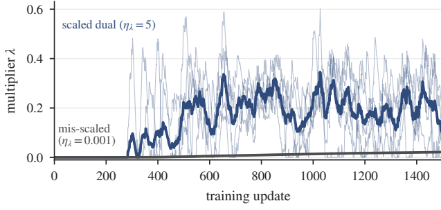
Figure 2: The Lagrange multiplier over training. Thick lines are five-seed means and thin lines the individual seeds.
