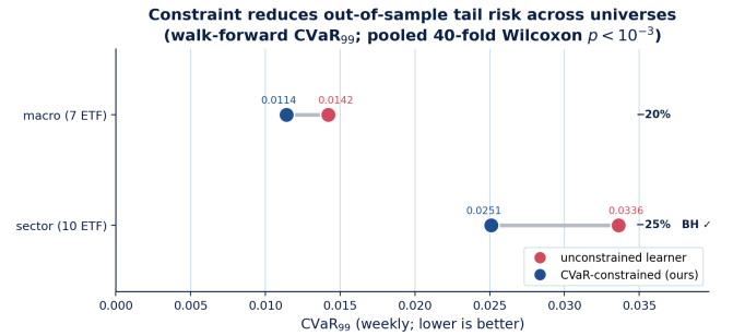
Figure 3: The constraint's robust win. Out-of-sample (walk-forward) CVaR 99 for the unconstrained learner (red) versus the CVaR-constrained learner (blue) on each universe. Arrow length is the tail-risk reduction. The reduction survives walk-forward on both universes (macro-ETF p = 0.0077 , sector p = 0.0003 , pooled 40-fold p = 8.8 \times 10^{-6} ), with Benjamini–Hochberg correction passing on both.
