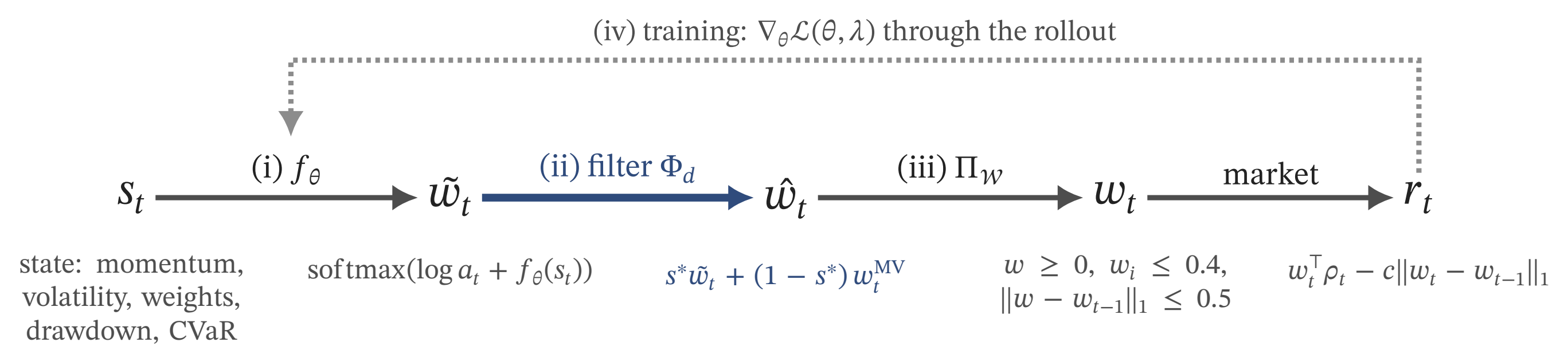
Figure 6. The decision at week t as a composition of maps.
