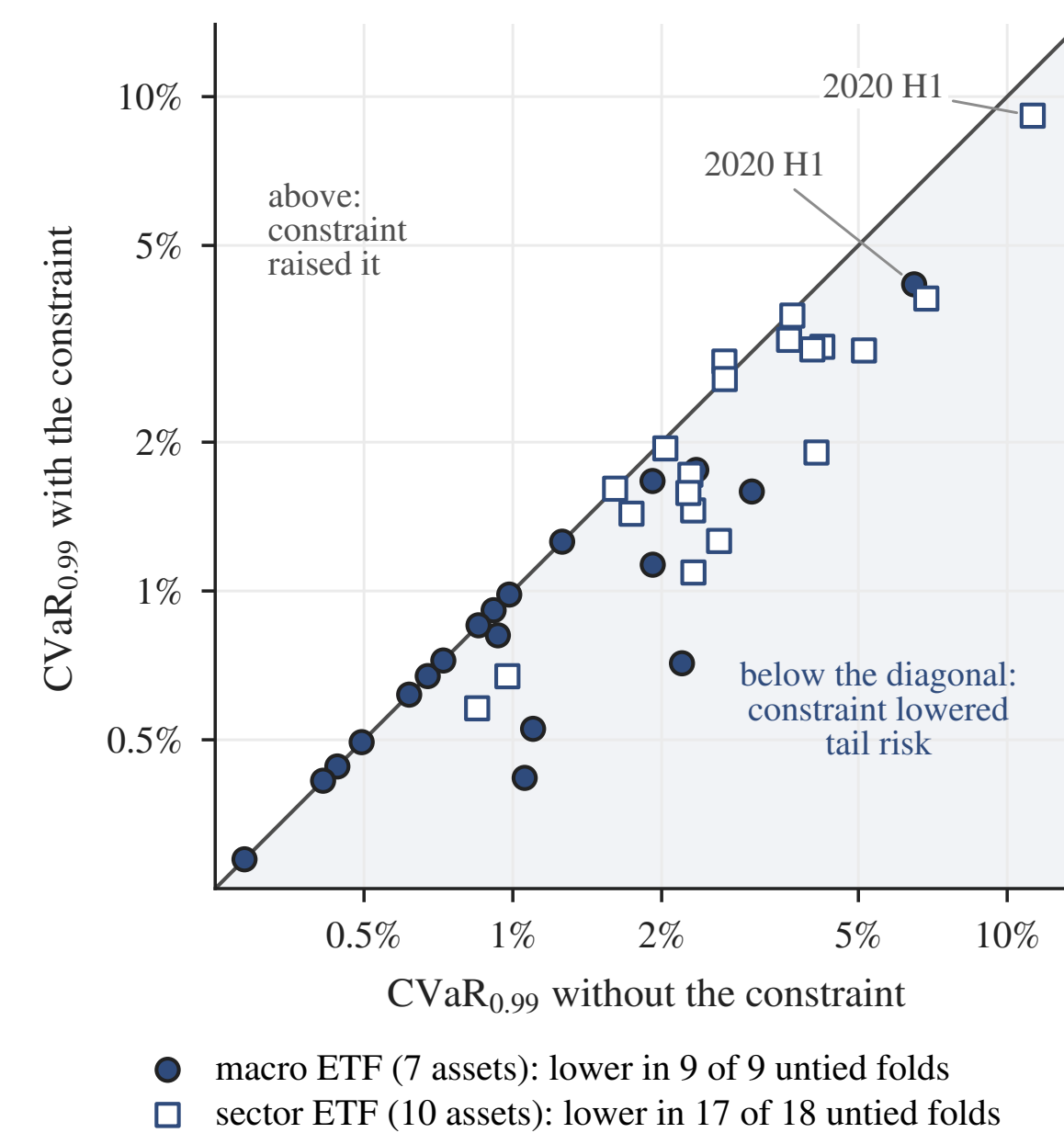
Figure 7. Walk-forward folds, CVaR 0.99 without against with the constraint (log scale). The largest reductions came in the first half of 2020.
