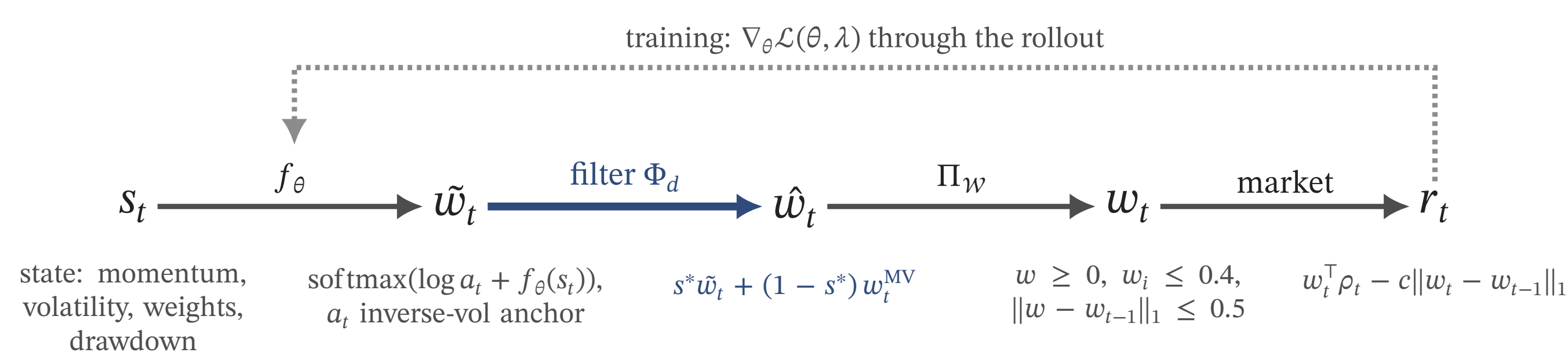
Figure 3. The decision at week t as a composition of maps. The navy map is the decision-time filter.
