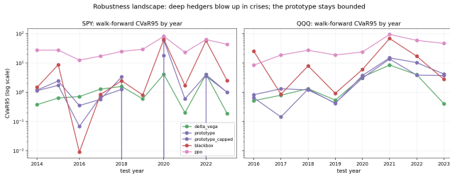
Figure 4: Robustness landscape. Walk-forward CVaR 95 by fold-year (log scale), both markets. PPO blows up in every crisis fold on both markets. The prototype stays bounded. The prototype’s known failure is the COVID-2020 fold. The volatility-scaled cap reduces this from 60.0 to 18.0.
