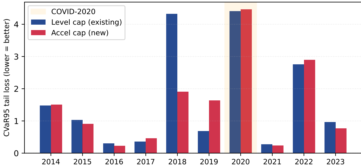
Regime-conditional cap: level vs acceleration (prototype, SPY, walk-forward)
