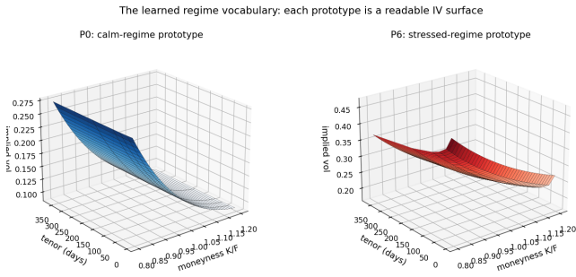
Figure 5: The model’s learned regime vocabulary. Each prototype reconstructs to a concrete implied-volatility surface. A low-level, gently sloped surface (left) is the calm-regime prototype. A high-level, steep surface (right) is the stressed one. This is the object the hedge keys on, and the explanation is the decision.
