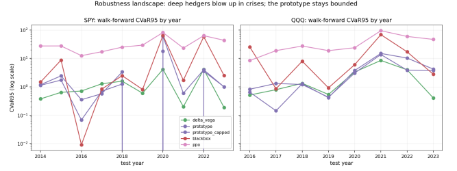
Figure 4: Robustness landscape. Walk-forward CVaR 95 by fold-year (log scale), both markets. PPO blows up in every crisis fold on both markets. The prototype stays bounded. The prototype’s known failure is the COVID-2020 fold. The volatility-scaled cap reduces this from 60.0 to 18.0.
