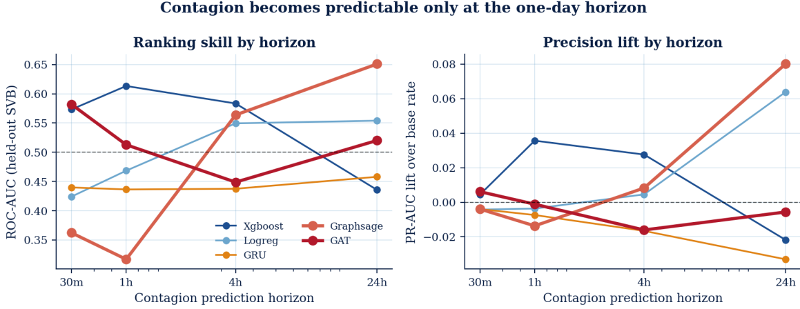
Figure 3: Lead-time (single-seed run). The left panel shows ranking skill (ROC-AUC) versus horizon; ROC-AUC is noisy at short horizons and only at 24h does GraphSAGE pull clearly ahead (0.65). The right panel shows precision lift over the base rate: every model stays near zero lift below 24h, where skill first emerges.
