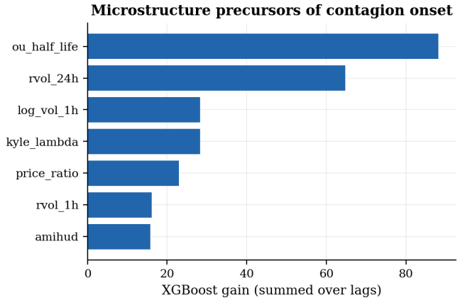
Figure 7: Which signals predict contagion onset (XGBoost gain, summed over lags). Mean-reversion speed (OU half-life) and recent volatility dominate, economically sensible fragility signals.
