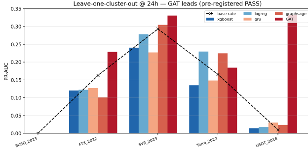
Figure 6: Leave-one-cluster-out PR-AUC at 24h. Graph models (GAT, dark red) lead the tabular baseline on the contagion-bearing folds; the single-positive USDT-2018 fold is a high-variance outlier we report but do not lean on.
