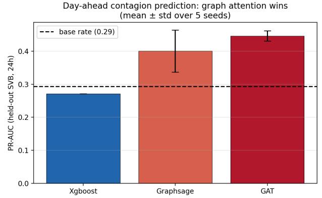
Figure 5: Day-ahead contagion prediction on the held-out SVB cluster, mean \pm std over five seeds. Graph attention (GAT) clears the base rate by a wide, stable margin; XGBoost sits on it.
