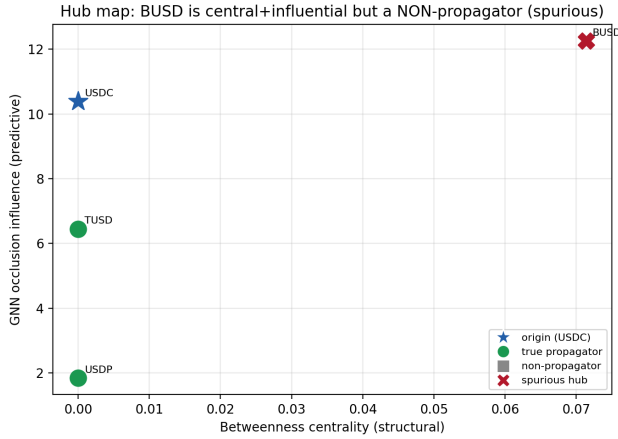
Figure 8: Exported hub map for USDC/SVB: graph betweenness (x) versus GNN influence (y), with the origin (USDC) marked separately. The top-ranked hub (BUSD) is the actionable output handed to causal analysis—where it is, surprisingly, refuted.
