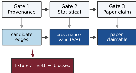
(b) Provenance-gated claim pipeline
