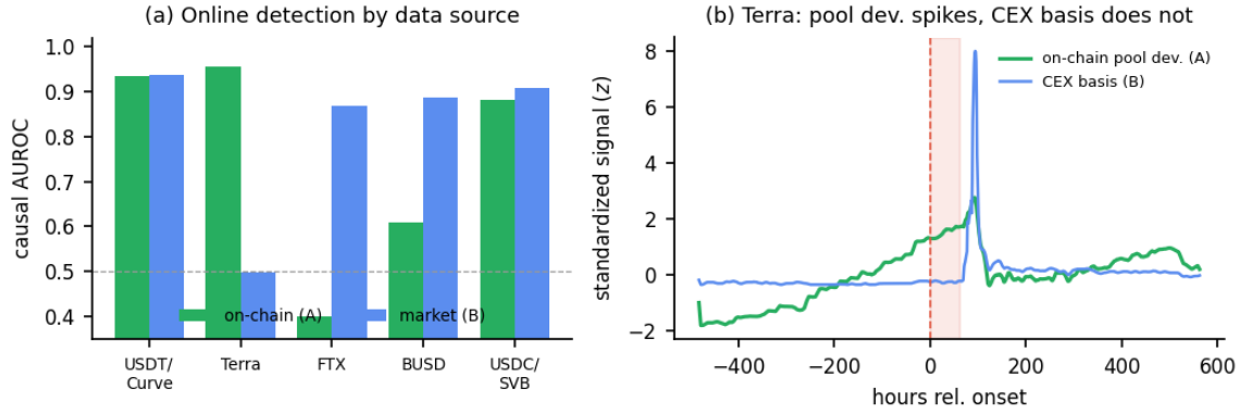
Figure 4: Online stress detection: Tier-A on-chain versus Tier-B market data. (a) Causal AUROC by data source. One unsupervised HMM, scored on its filtered (forward-only) posterior, run separately on on-chain pool state (green) and market state (blue). On-chain wins or ties for the three pool-borne events and is decisive for Terra; market wins for the exchange-/regulation-borne FTX and BUSD — complementary layers, not a single winner. (b) Why, for Terra. Standardised on-chain pool deviation rises through the panic window (shaded) while the USDT/Binance basis stays flat: USDT held its peg during a UST de-peg, so a market-only monitor is blind to the crisis.
