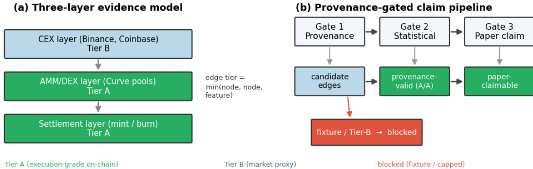
Figure 2: Evidence model and provenance-gated claim pipeline. (a) Stress is represented as a directed graph over three layers: centralized-exchange (CEX) market nodes (Tier B, market-proxy), on-chain AMM/DEX pool nodes and settlement (mint/burn) nodes (Tier A, execution-grade). Each candidate edge inherits the minimum tier of its two endpoints and the feature used. (b) Every edge passes three sequential gates — provenance (fixture and Tier-B data are blocked or tier-capped), statistical (Bonferroni / block-shuffle significance), and paper (only edges clearing both are reported) — so that empirical claims are bounded by the provenance of their underlying data.
