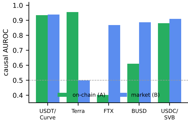
(a) Online detection by data source
