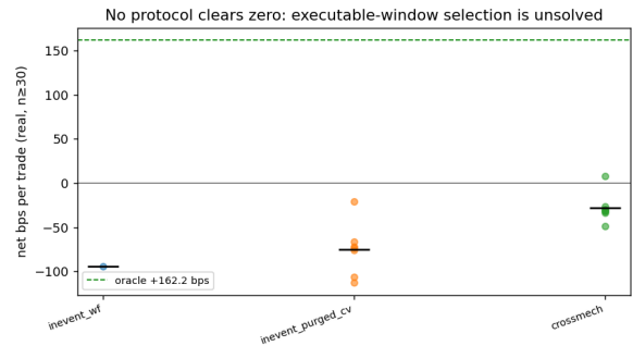
Figure 7: The CEX selection null, visualised. Each point is one of the 81 pre-registered paths (well-defined, n \geq 30 ); the bar is the per-protocol mean. Every protocol sits below zero and far below the oracle ceiling, including the in-distribution purged cross-validation—no configuration selects profitable executable windows on the CEX order book.
