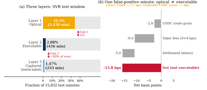
Figure 2: (a) Three-layer framework for the SVB test window (15,832 min). Layer 1 optical (34.3%), Layer 2 executable (2.88%), Layer 3 captured by cross-mechanism meta-labeling (1.47%). Gap 1 (12×) is a measurement problem. Gap 2 is a training problem. (b) Worked example. A minute that appears profitable on the chart nets -15.8 bps after VWAP book-walking, fees, and route-direction mismatch.
