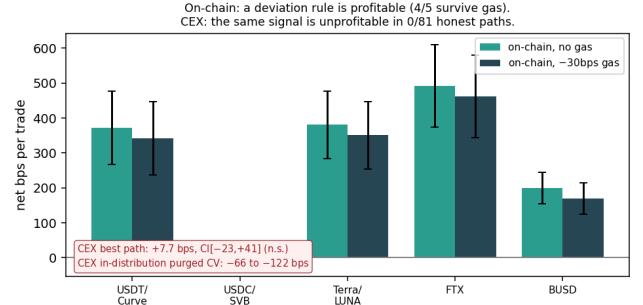
Figure 6: Venue specificity. On the on-chain Curve venue a model-free deviation rule is profitable in every episode (four of five survive a 30 bps gas haircut); on the CEX order book the same signal is unprofitable in 0/81 honest paths and strongly negative even under in-distribution purged cross-validation. The optical-to-executable barrier is a property of CEX order-book microstructure, not of stablecoin depegs.
