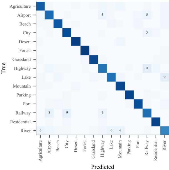
Stacking (balanced)
