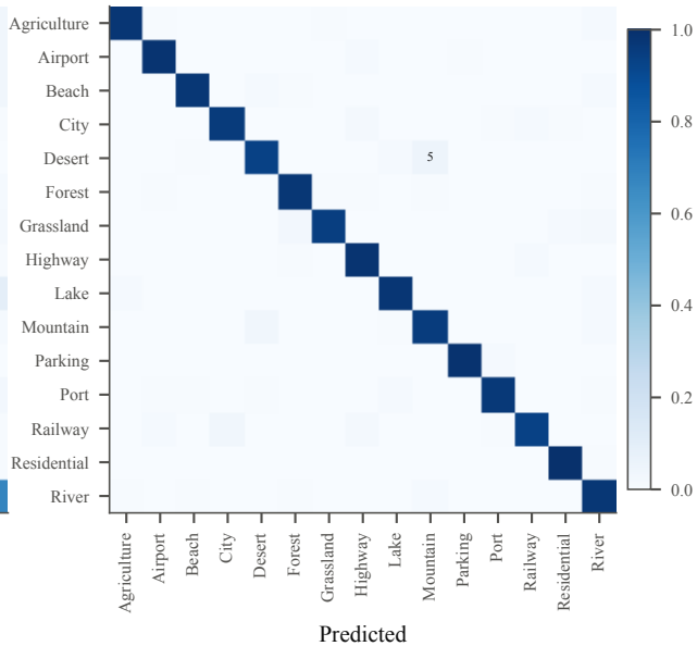
EfficientNet-B3 (balanced)
