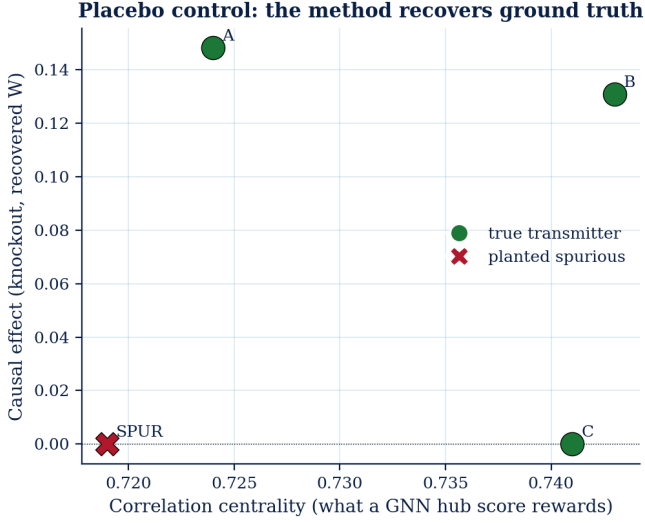
Figure 4: Placebo control on synthetic data. A planted spurious co-mover (SPUR) is correlationally central but causally inert. The knockout recovers the true transmitters.
