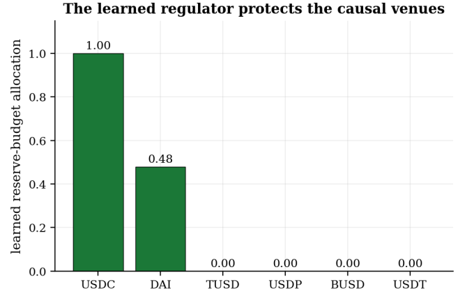
Figure 11: A PPO regulator, given only the network and no causal labels, learns to protect the causal venues (USDC, DAI) and allocate nothing to the spurious hub (BUSD).
