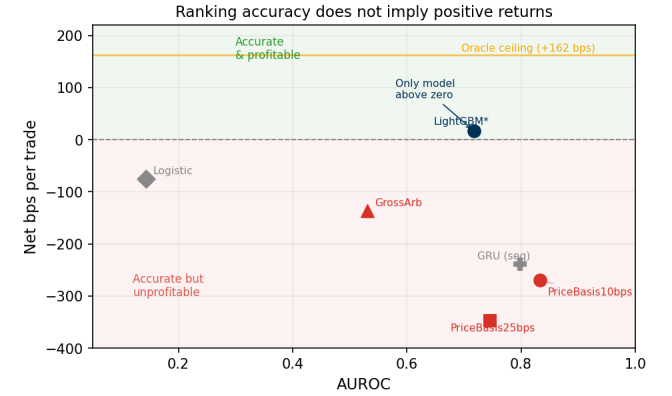
Figure 4: AUROC vs. net bps per trade for all models. The right quadrant is dominated by models that rank windows correctly but trade the wrong ones. PriceBasis10bps (AU- ROC 0.83) loses −270 bps; LightGBM (AUROC 0.72, navy) is the only non-oracle model above zero. High ranking accu- racy is necessary but not sufficient for profitability.
