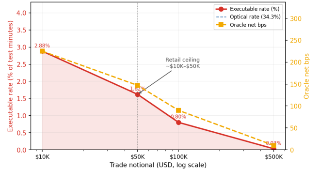
Figure 3: Notional scaling (SVB test split). The executable rate collapses from 2.88% at $10K to 0.03% at $500K: book depth, not fees, is the binding institutional constraint.
