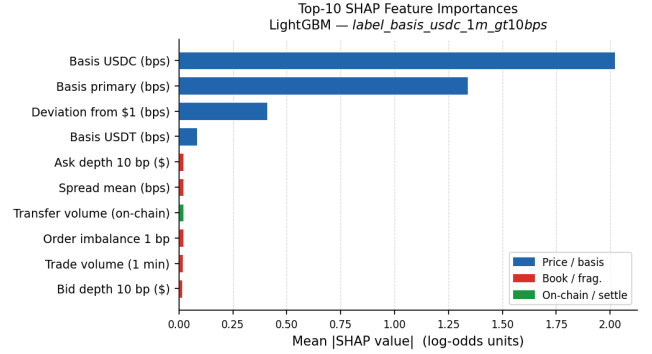
Figure 4: SHAP feature importance (mean |SHAP| ) for LightGBM on the full feature set. Price features (navy, 94.8%); book+fragmentation (red, 3.4%); settlement (green, 1.8%). Depth-imbalance features provide the marginal microstructure lift.
