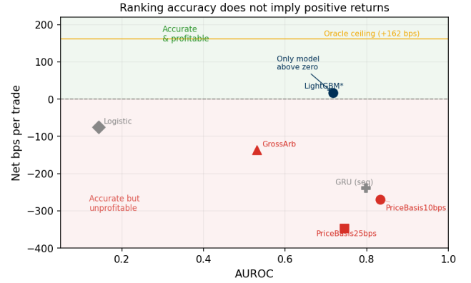
Figure 4: AUROC vs. net bps per trade for all models. The right quadrant is dominated by models that rank windows correctly but trade the wrong ones. PriceBasis10bps (AUROC 0.83) loses -270 bps; LightGBM (AUROC 0.72, navy) is the only non-oracle model above zero. High ranking accuracy is necessary but not sufficient for profitability.
