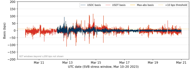
Figure 2: Cross-quote basis during the SVB test window (Mar 10–20 2023). USDC basis (navy) exceeds 10 bps in 12.4% of minutes, USDT basis (red) in 27.4%, and max-abs basis (gold) in 34.3%. The price-to-execution ratio is 12 \times .
