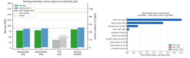
Figure 5: Oracle capture across four training conditions (Terra/LUNA only, Celsius/3AC only, FTX only, All four pooled).
