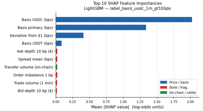
Figure 5: SHAP feature importance (mean |\text{SHAP}| ) for LightGBM. Price features (navy, 94.8%): USDC cross-quote basis and primary basis dominate. Book+fragmentation (red, 3.4%): ask-side depth at 10 bps (mean |\text{SHAP}|=0.021 , rank 5) and bid-ask spread (rank 6). Settlement proxies (green, 1.8%).
