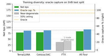
Figure 7: Oracle capture across four training conditions. Dashed: 50% ceiling; hatched: FTX near-degenerate.
