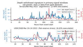
Figure 8: Depth withdrawal signature (real L2). Ask depth (blue) collapses and spread (red) widens identically across Terra/LUNA and SVB stress despite different triggers.
