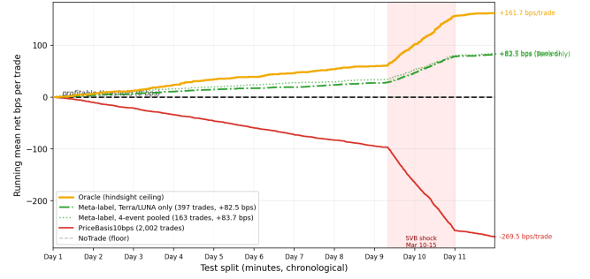
Figure 6: No calm-trained model ever crosses zero. Meta-labeling trained on a structurally different event (Terra/LUNA) is the only approach that achieves positive returns, earning +82.5 bps—roughly half the oracle’s +161.7 bps. Every other learned model loses money despite sometimes high AUROC. Oracle (gold); meta-label Terra/LUNA only (green solid); meta-label 4-event pooled (green dotted); PriceBasis10bps (red); NoTrade (grey dashed). Shaded: SVB shock window.
