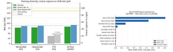
Figure 5: Oracle capture across four training conditions (Terra/LUNA calibration, SVB test). Dashed: 50% ceiling; hatched: FTX near-degenerate (1 trade).
