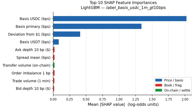
Figure 5: SHAP feature importance (mean |\text{SHAP}| ) for LightGBM. Price features (navy, 94.8%): USDC cross-quote basis and primary basis dominate. Book+fragmentation (red, 3.4%): ask-side depth at 10 bps (mean |\text{SHAP}|=0.021 , rank 5) and bid-ask spread (rank 6). Settlement proxies (green, 1.8%).
