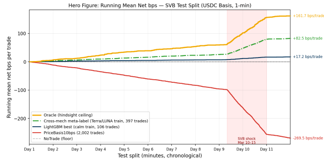
Figure 3: Hero figure: running mean net bps per trade (USDC/SVB test split). Five strategies span the full per- formance range. Oracle (gold): +161.7 bps/trade. Cross- mech meta-label (green dash-dot, Terra/LUNA train): +82.5 bps. LightGBM best (navy, calm train): +17.2 bps. PriceBasis10bps (red): −269.5 bps. NoTrade (grey dashed): 0 bps. The shaded region marks the SVB shock (Day 10–11), where the price rule accumulates its steepest losses while the oracle and meta-label remain profitable.
