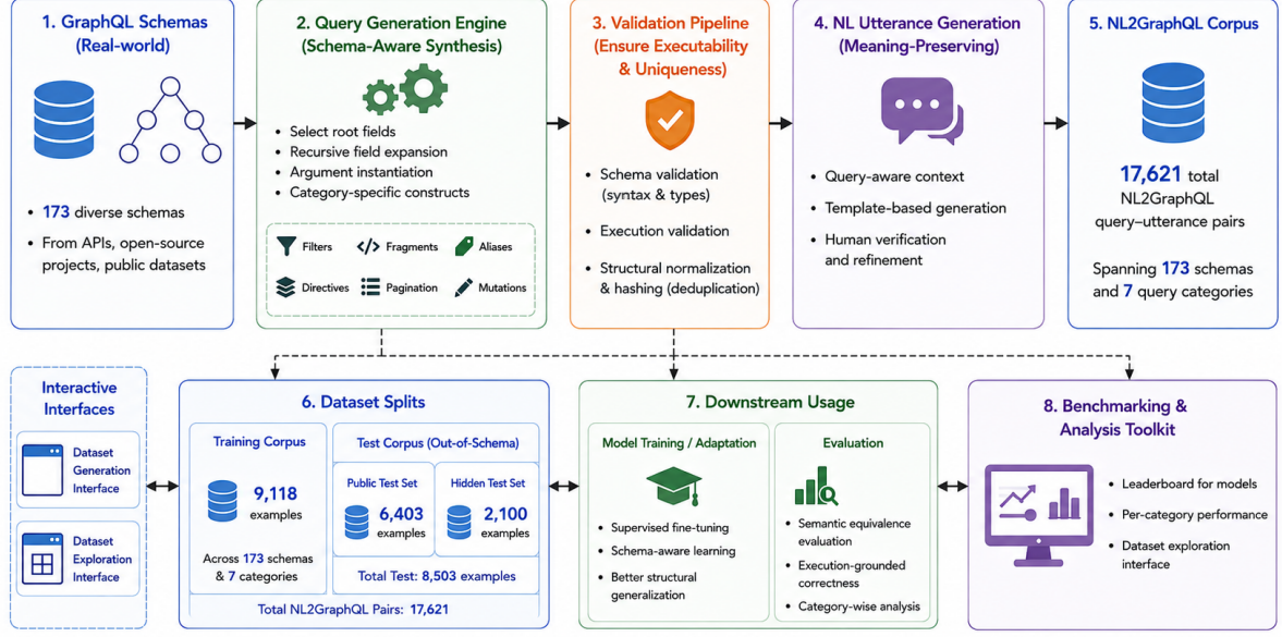
Figure 2: Overview of the proposed AutoGraphQL framework.
