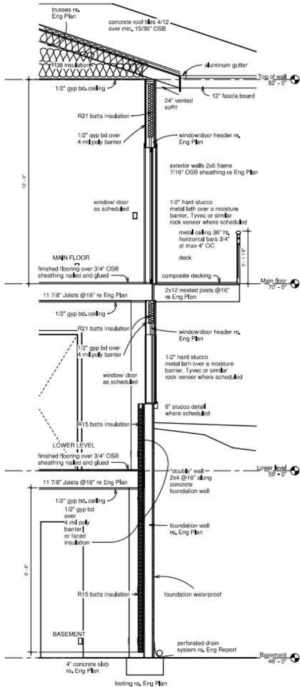
1 Callout of Section A 1/2" = 1'-0"
