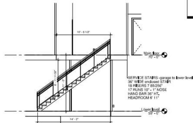
3 Section C service stairs 1/4" = 1'-0"
