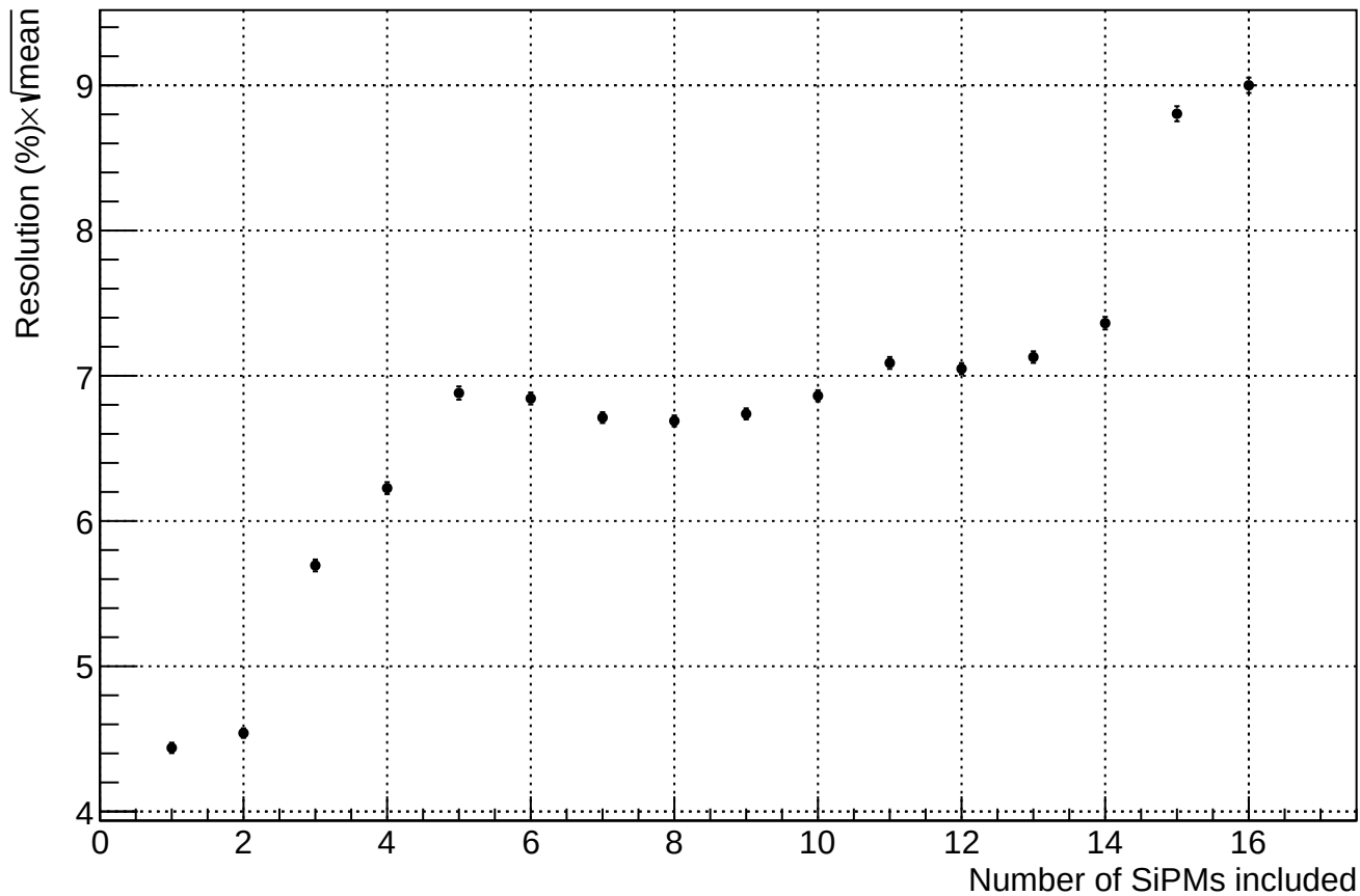
Resolution \times \sqrt{\text{mean}} vs number of included SiPMs
