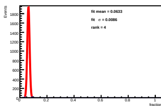
SIPM 08 fraction of full 16-SIPM sum
