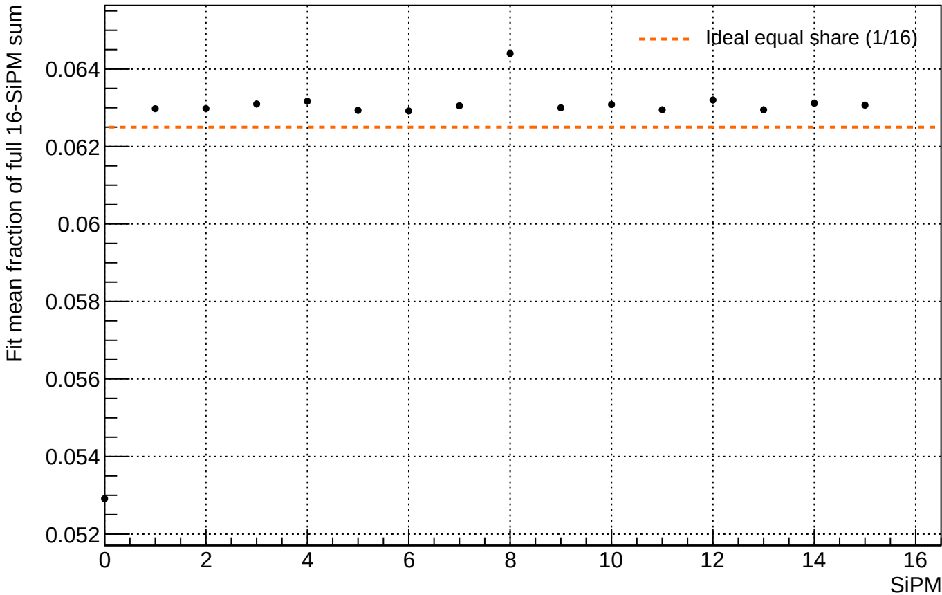
Fit mean fraction collected by each SiPM
