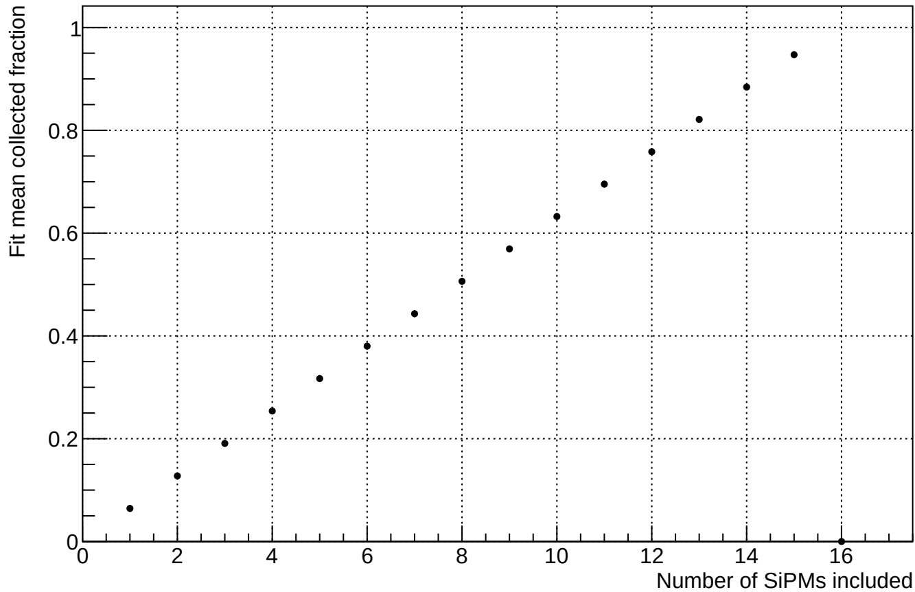
Fit mean cumulative fraction vs number of SiPMs
