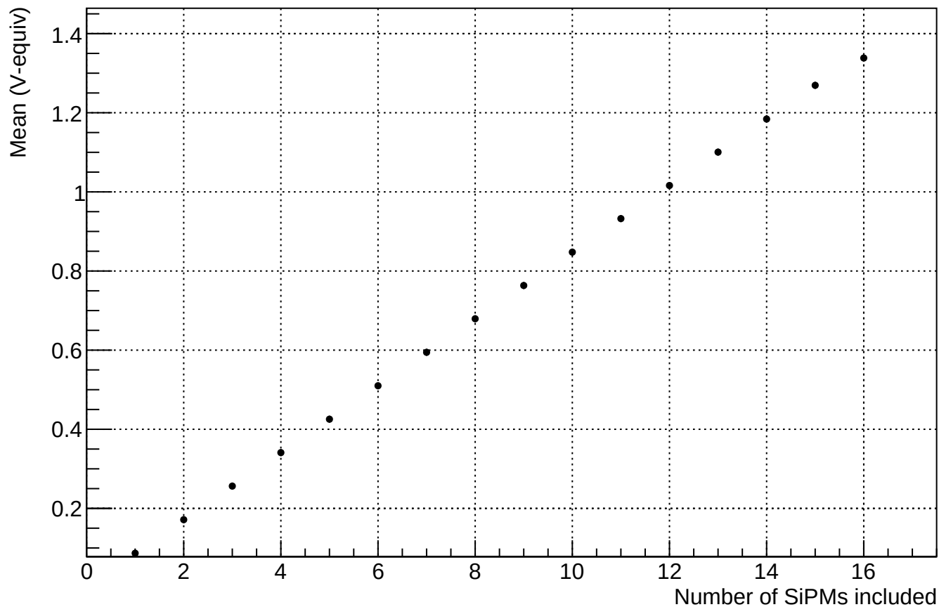
Mean reconstructed central signal vs number of included SiPMs
