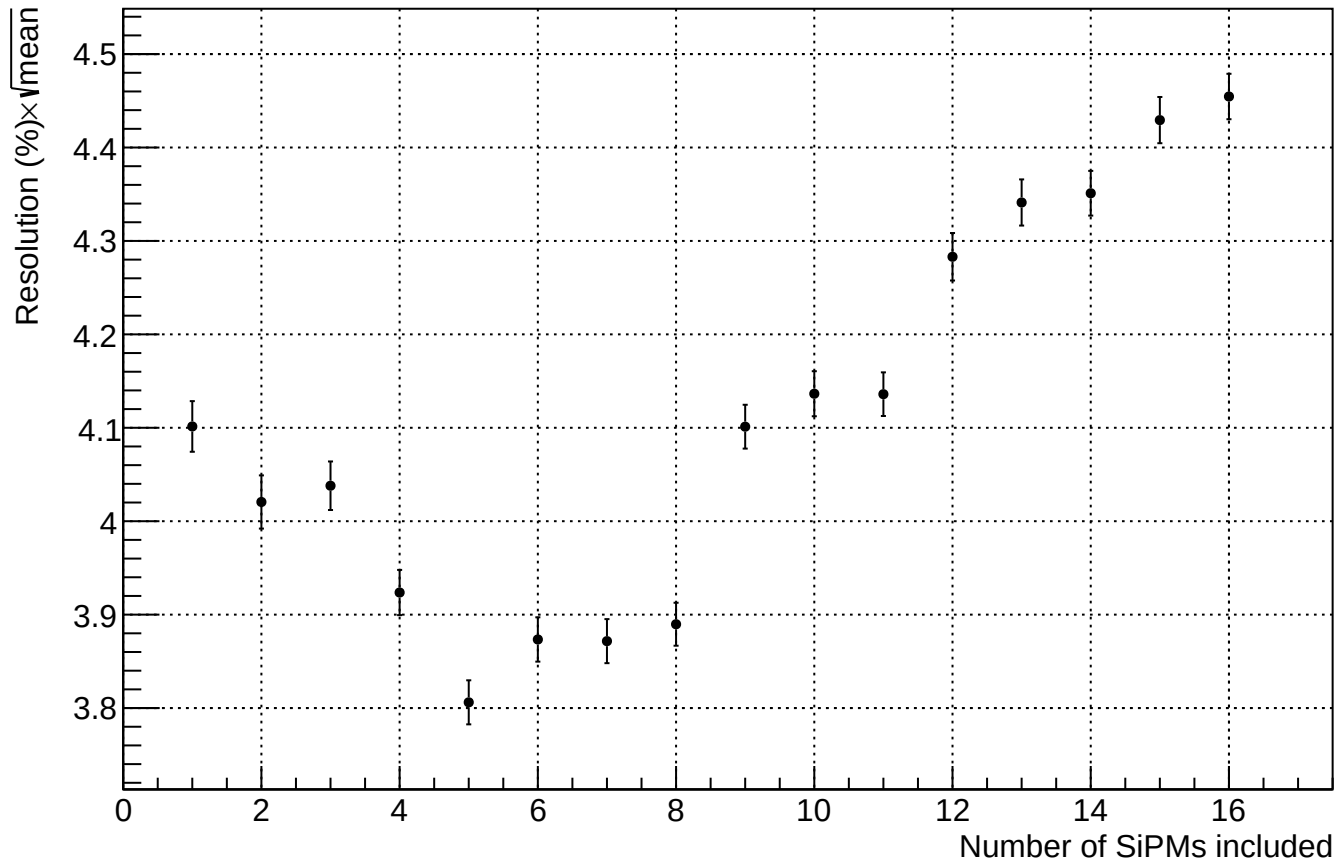
Resolution \times \sqrt{\text{mean}} vs number of included SiPMs
