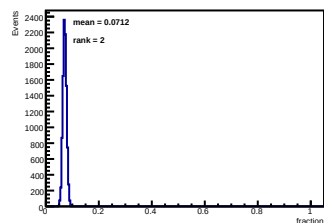
SiPM 05 fraction of full 16-SiPM sum
