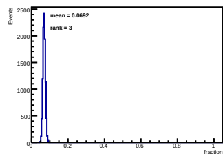
SiPM 01 fraction of full 16-SiPM sum
