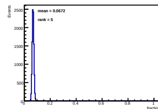
SiPM 07 fraction of full 16-SiPM sum
