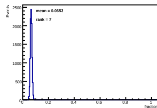
SiPM 02 fraction of full 16-SiPM sum
