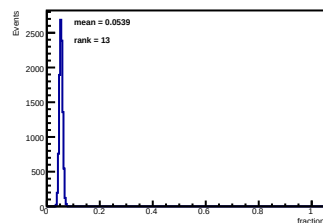
SiPM 06 fraction of full 16-SiPM sum
