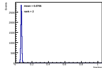
SiPM 09 fraction of full 16-SiPM sum
