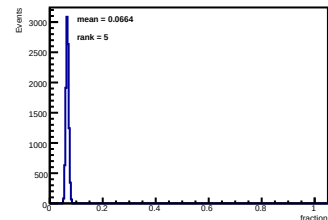
SiPM 11 fraction of full 16-SiPM sum
