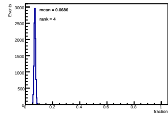
SiPM 05 fraction of full 16-SiPM sum
