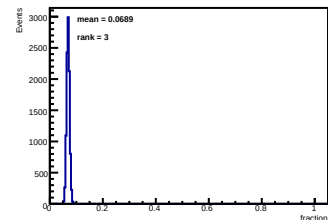
SiPM 13 fraction of full 16-SiPM sum
