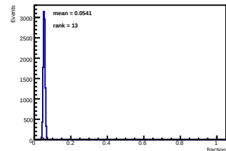
SiPM 10 fraction of full 16-SiPM sum
