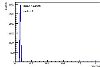
SiPM 06 fraction of full 16-SiPM sum
