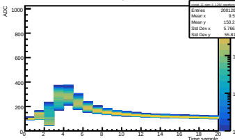
Run 039 Vol 1.26V | Crystal 12 SiPM 0
