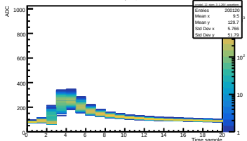
Run 039 Vol 1.26V | Crystal 12 SiPM 3
