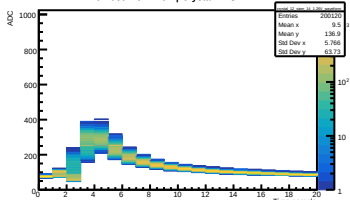
Run 039 Vol 1.26V | Crystal 12 SiPM 14
