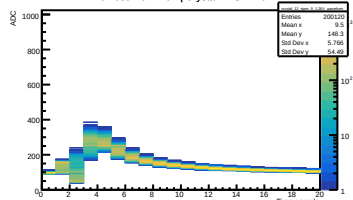
Run 039 Vol 1.26V | Crystal 12 SiPM 9
