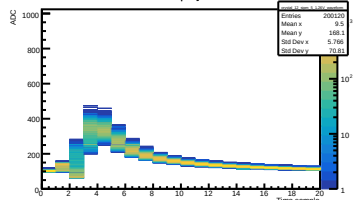
Run 039 Vol 1.26V | Crystal 12 SiPM 5
