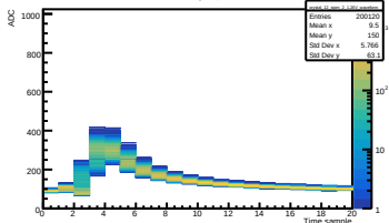
Run 039 Vol 1.26V | Crystal 12 SiPM 2
