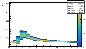
Run 039 Vol 1.26V | Crystal 12 SiPM 15
