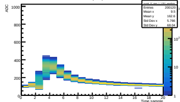
Run 039 Vol 1.26V | Crystal 12 SiPM 1
