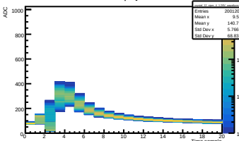
Run 039 Vol 1.26V | Crystal 12 SiPM 4
