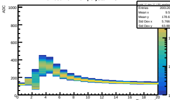
Run 039 Vol 1.26V | Crystal 12 SiPM 12
