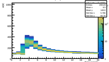
Run 039 Vol 1.26V | Crystal 12 SiPM 7
