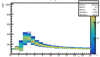
Run 039 Vol 1.26V | Crystal 12 SiPM 10
