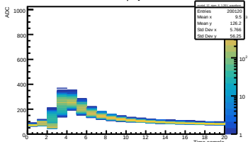
Run 039 Vol 1.26V | Crystal 12 SiPM 6
