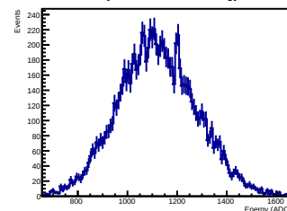
Crystal 12 SIPM 15 Energy
