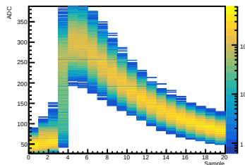
Crystal 12 SiPM 02 Waveform
