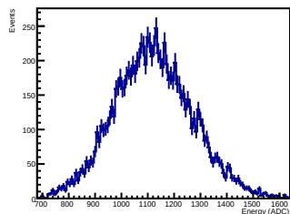
Crystal 12 SIPM 09 Energy
