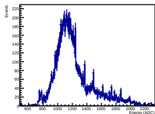
Crystal 12 SIPM 05 Energy
