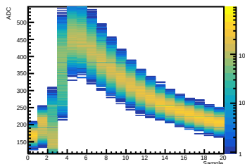
Crystal 12 SiPM 05 Waveform
