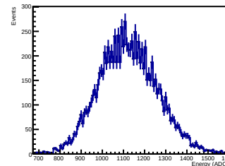
Crystal 12 SIPM 11 Energy
