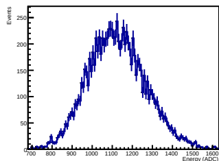
Crystal 12 SIPM 10 Energy
