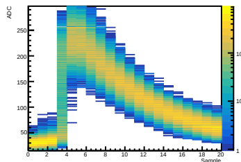
Crystal 12 SiPM 03 Waveform
