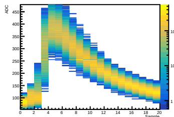
Crystal 12 SiPM 11 Waveform
