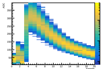
Crystal 12 SiPM 04 Waveform
