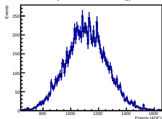
Crystal 12 SIPM 14 Energy
