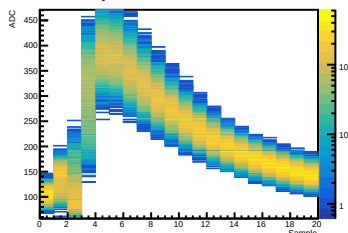
Crystal 12 SiPM 13 Waveform
