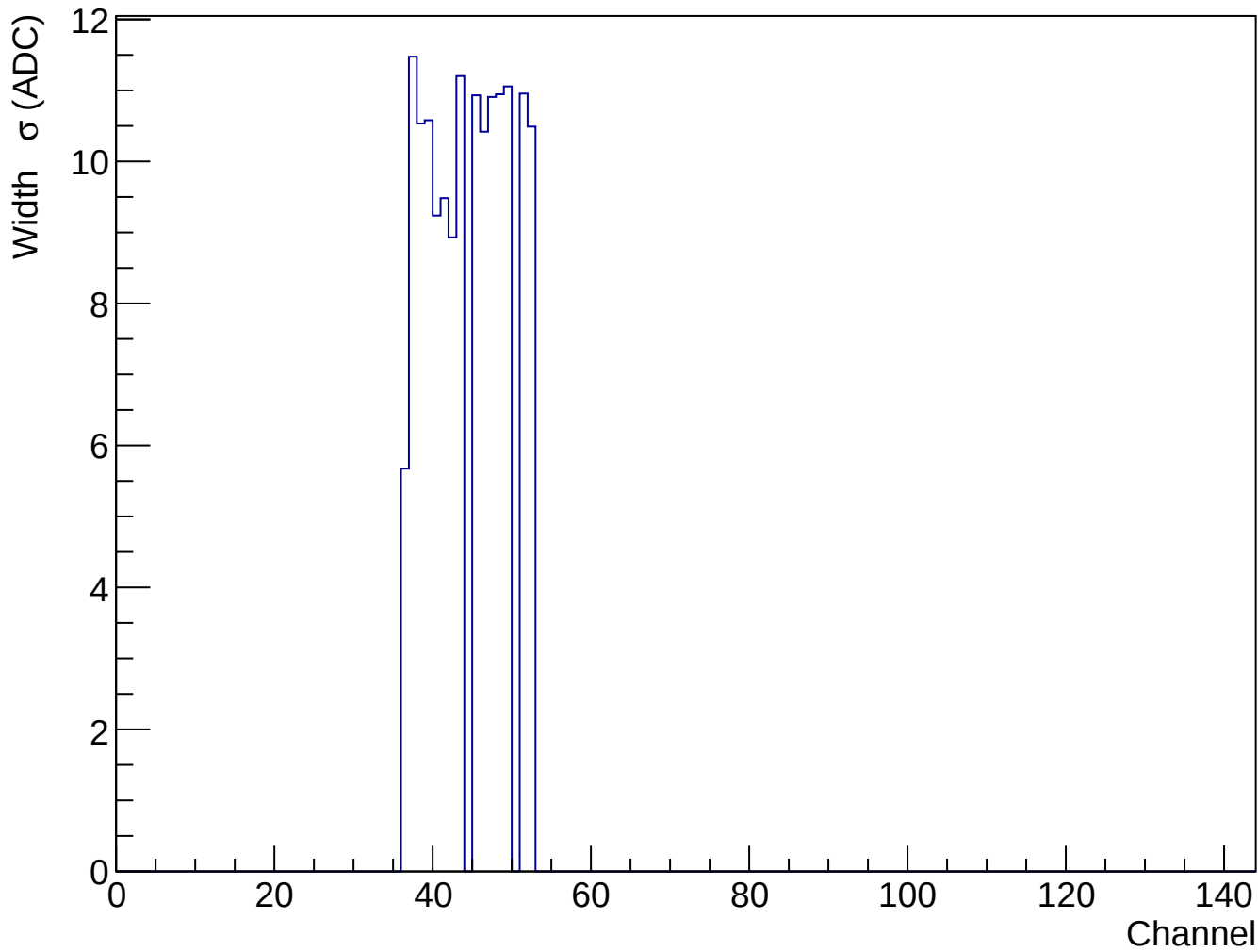
Pedestal Width ( \sigma ) vs Channel
