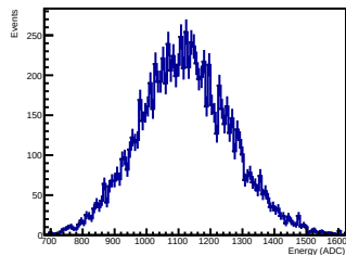
Crystal 12 SIPM 01 Energy
