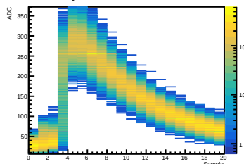
Crystal 12 SiPM 14 Waveform
