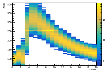
Crystal 12 SiPM 15 Waveform
