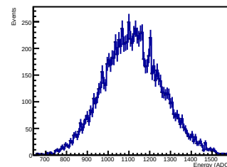
Crystal 12 SIPM 07 Energy
