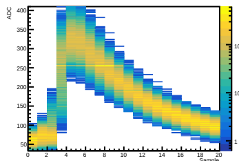
Crystal 12 SiPM 07 Waveform
