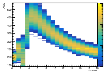
Crystal 12 SiPM 12 Waveform
