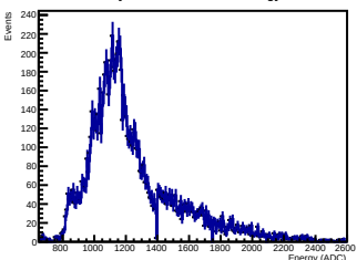
Crystal 12 SIPM 12 Energy
