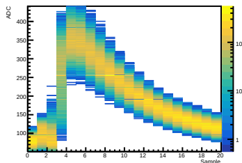
Crystal 12 SiPM 01 Waveform
