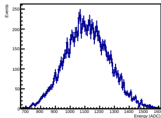
Crystal 12 SIPM 02 Energy
