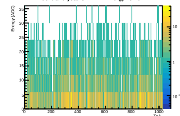
Central Crystal SIPM 12: Energy vs ToA
