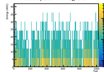
Central Crystal SIPM 10: Energy vs ToA
