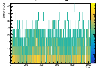
Central Crystal SIPM 12: Energy vs ToA
