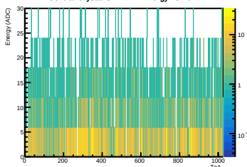
Central Crystal SIPM 12: Energy vs ToA
