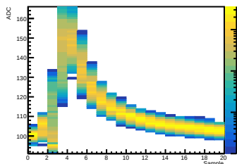
Crystal 12 SiPM 06 Waveform
