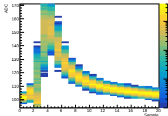
Crystal 12 SiPM 02 Waveform
