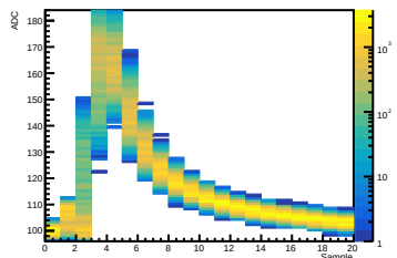
Crystal 12 SiPM 11 Waveform
