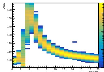
Crystal 12 SiPM 14 Waveform
