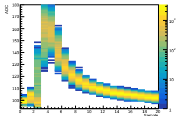
Crystal 12 SiPM 07 Waveform
